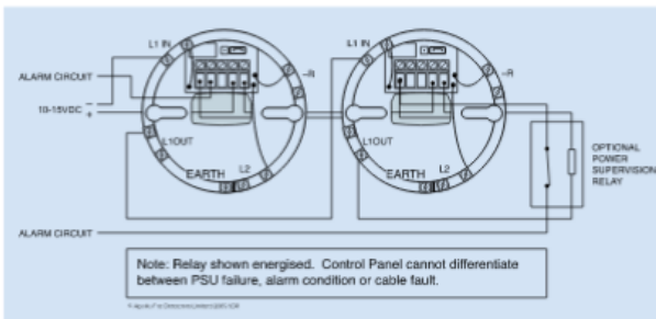
Fig.6 Wiring diagram of 12V Relay Base
